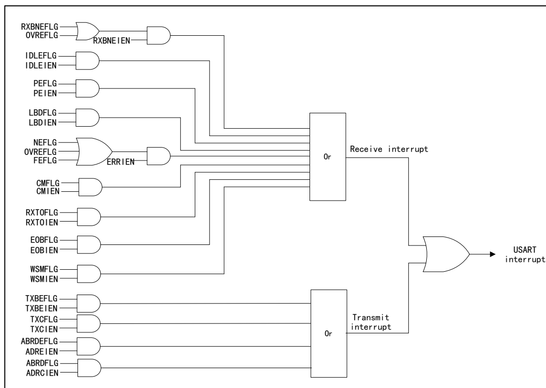
Figure 70 UART Interrupt Mapping
