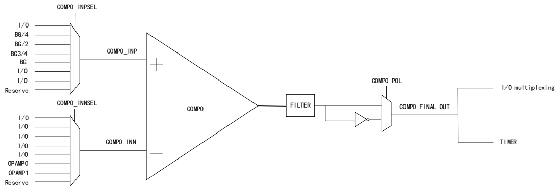
Figure 81 COMP0 Structure Block Diagram
