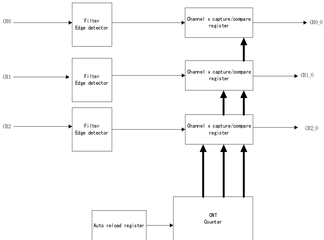
Figure 51 Structure Block Diagram
