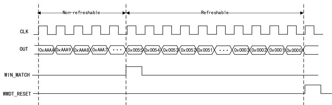
Figure 66 Timing Diagram
